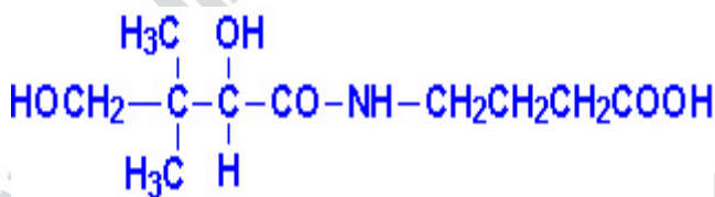
Figure: Structure of Pantothenic Acid
