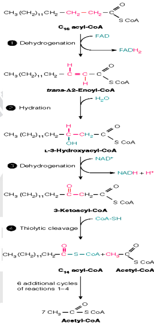
Fig 4.7: \beta -oxidation of fatty acid
