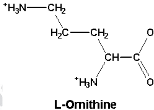
Fig 5.5: Non-Proteogenic Amino acids
