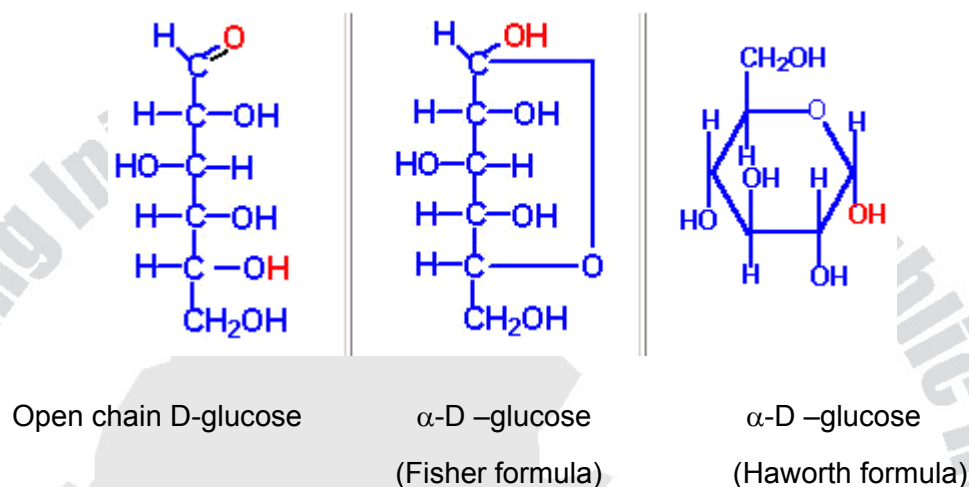
Fig.2.1. structures of D.Glucose
