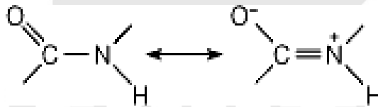
Fig 5.9: A peptide bond
