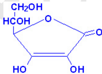
Figure: Structure of Ascorbic Acid
