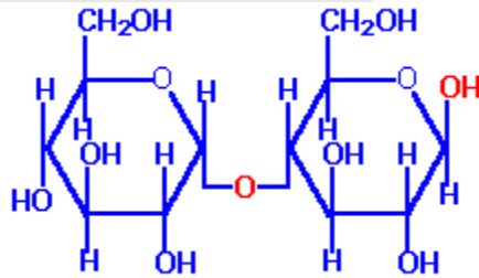
Fig 2.5. Structure of Maltose
