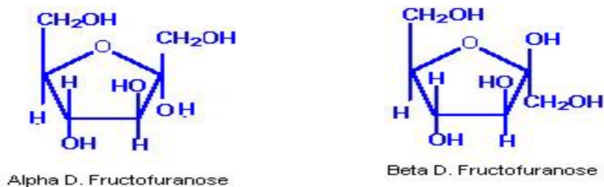
Fig 2.4. \alpha and \beta forms of Fructose
