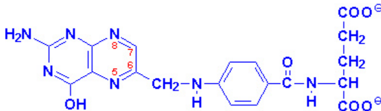
Figure: Structure of Folic Acid
